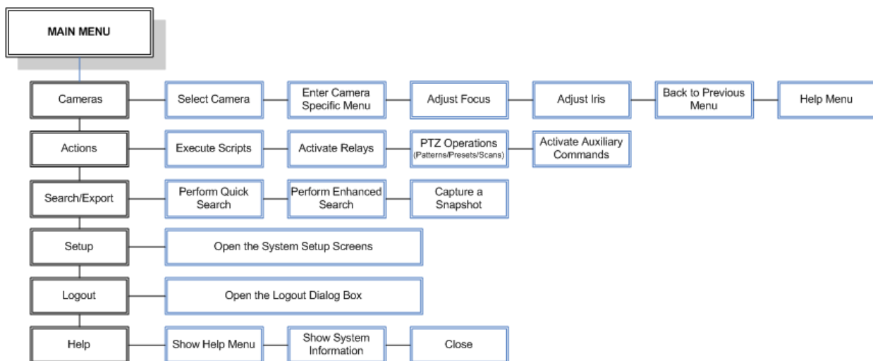
Figure 12. DVR5100 Menu Hierarchy
